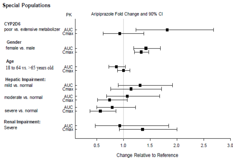
Figure 4: Effect of Intrinsic Factors on Aripiprazole Pharmacokinetics
